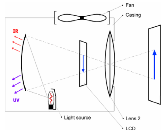
Fig. 4: Solution principle "Image Projection System"
